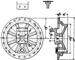
Figs. 922-925. Back Head. Cylinder Heads, Consolidation (2-8-0) Locomotive.
